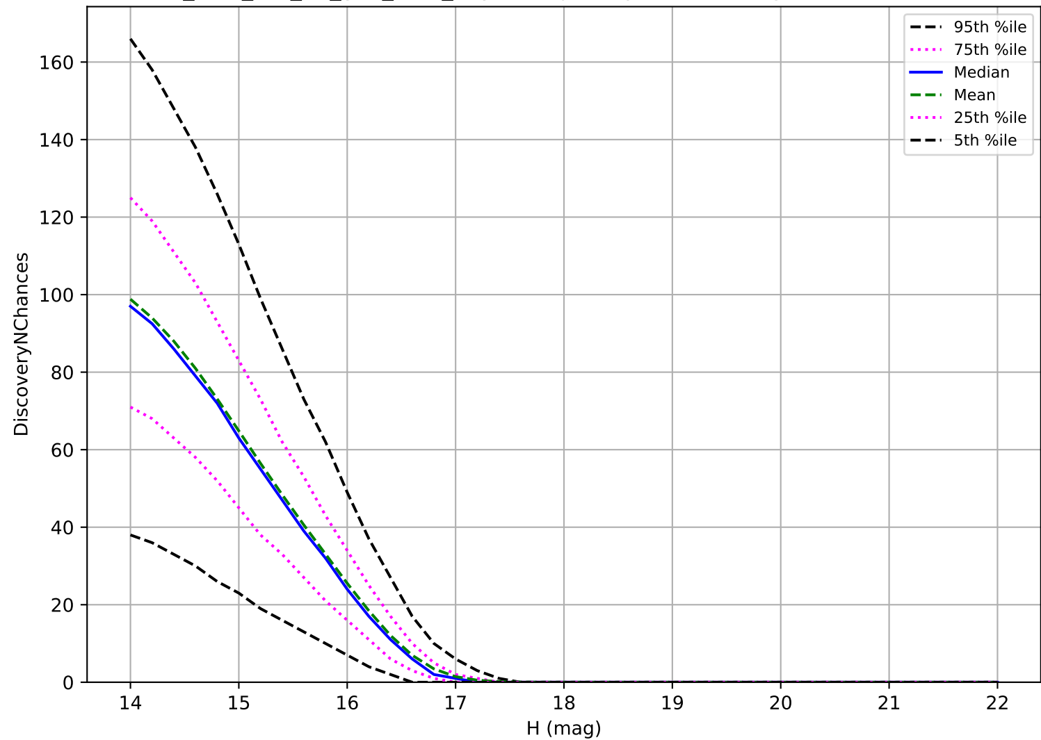
too_elab_r64_d3_griz_v3.4_10yrs: Trojan 3 pairs in 15 nights detection loss
