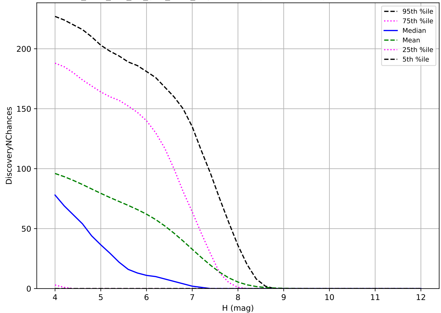
too_elab_r64_d3_griz_v3.4_10yrs: TNO 3 pairs in 15 nights detection loss
