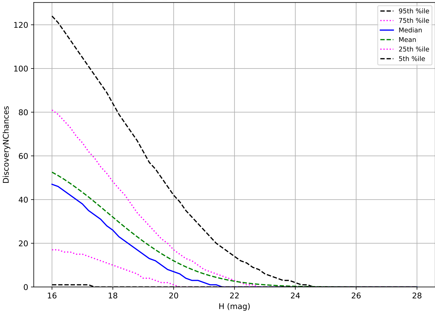
too_elab_r64_d3_griz_v3.4_10yrs: PHA 3 pairs in 15 nights detection loss
