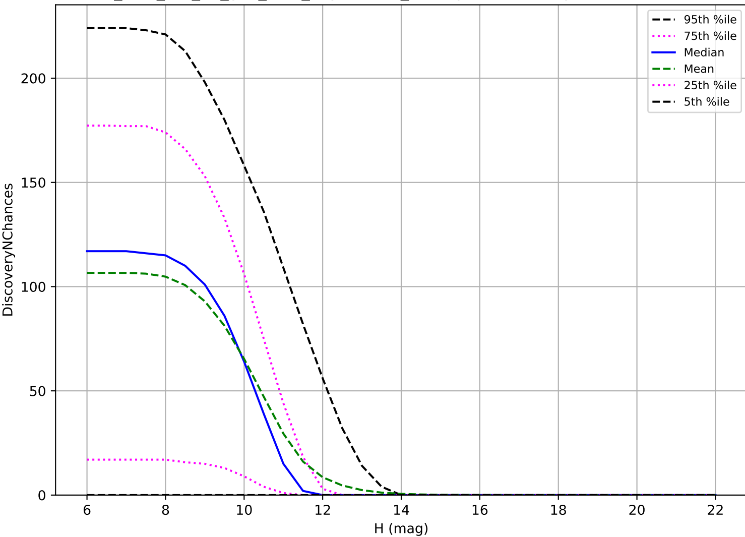
too_elab_r64_d3_griz_v3.4_10yrs: OCC_r20 3 pairs in 15 nights detection loss
