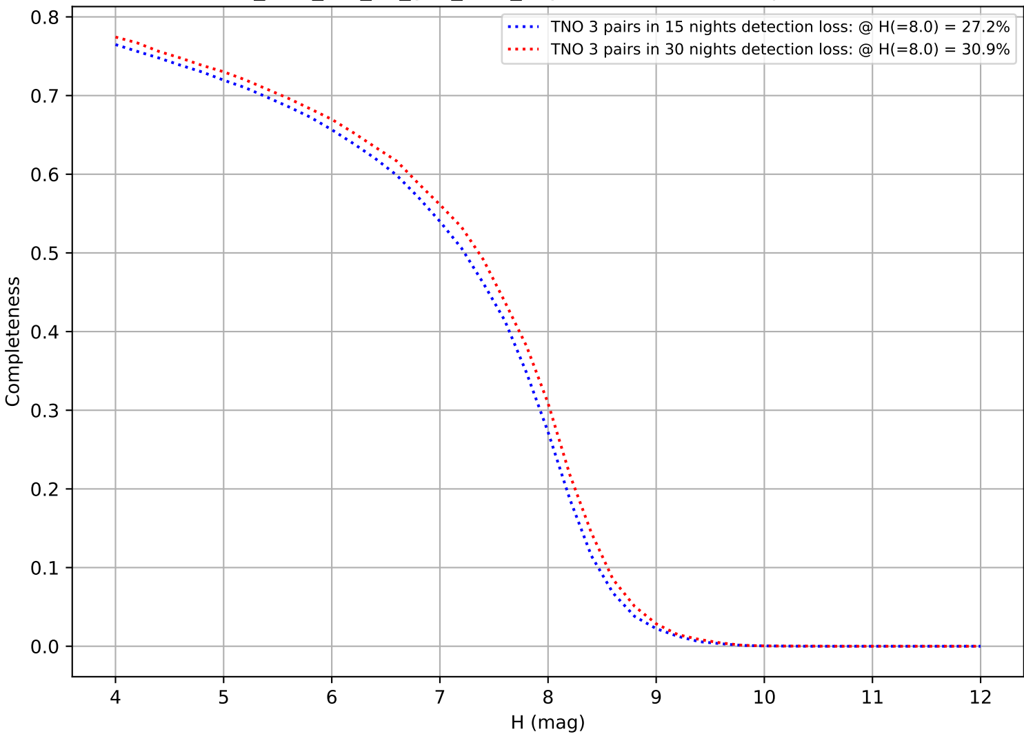
too_elab_r64_d3_griz_v3.4_10yrs: DifferentialCompleteness
