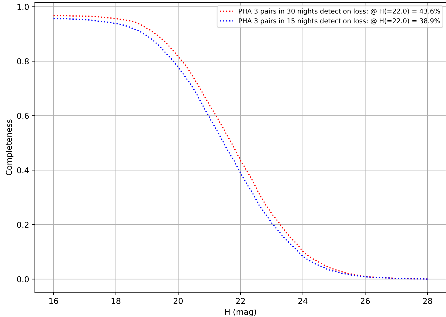
too_elab_r64_d3_griz_v3.4_10yrs: DifferentialCompleteness
