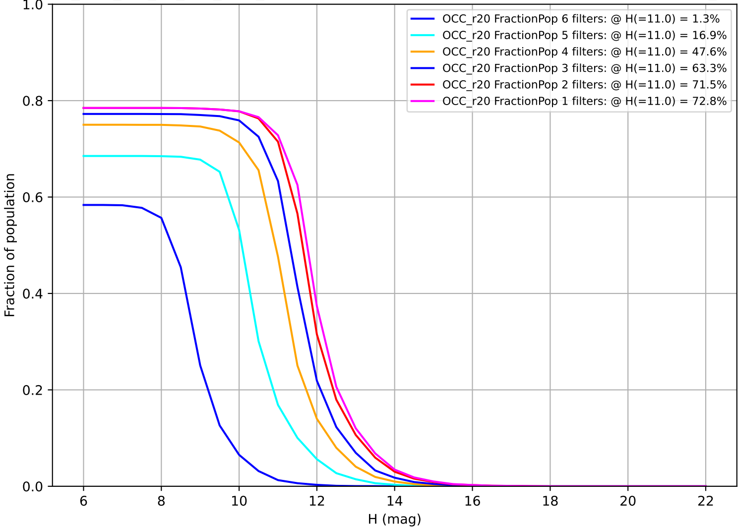
too_elab_r64_d3_griz_v3.4_10yrs: Fraction of population with colors in X filters OCC_r20
