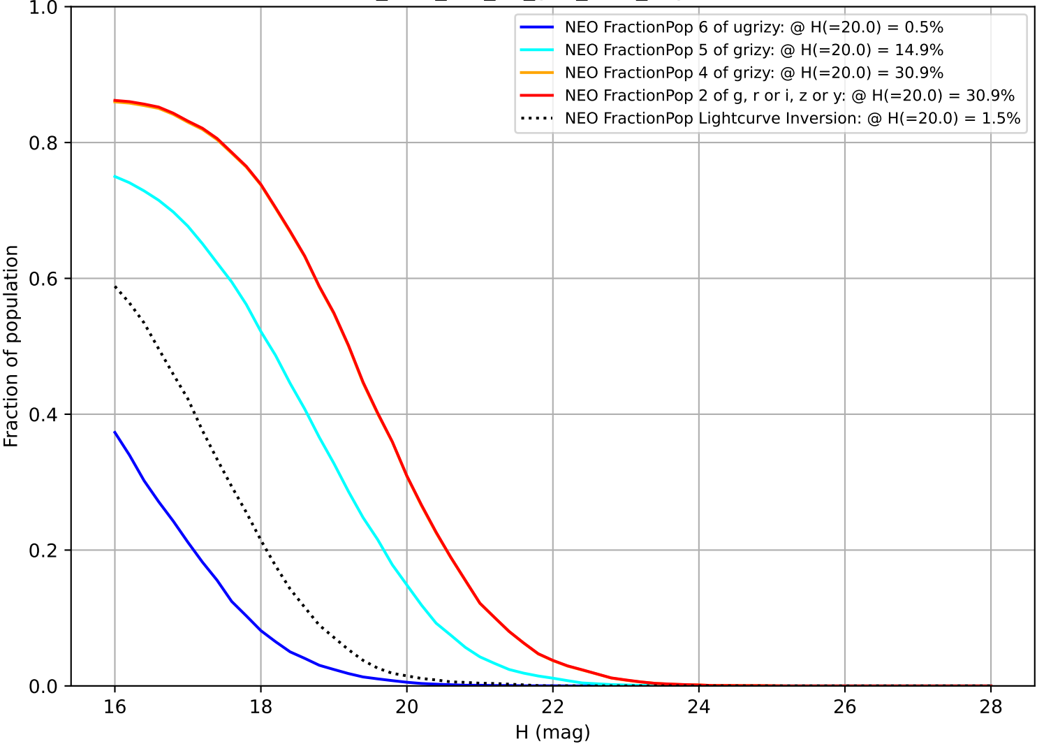
too_elab_r64_d3_griz_v3.4_10yrs NEO
