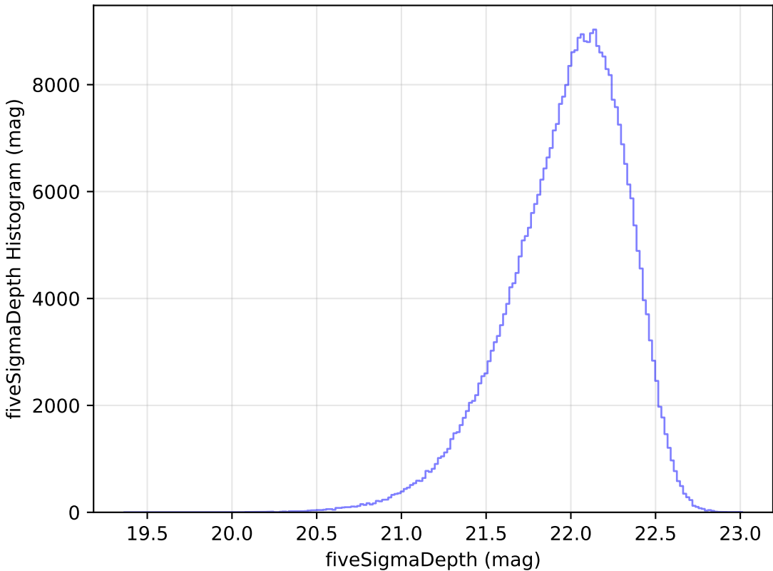
too_elab_r64_d3_griz_v3.4_10yrs y: fiveSigmaDepth Histogram
