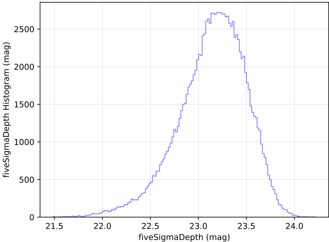
too_elab_r64_d3_griz_v3.4_10yrs u: fiveSigmaDepth Histogram
