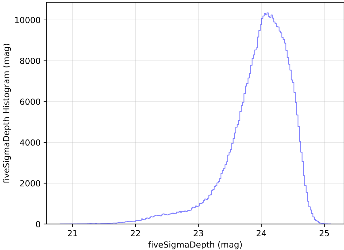
too_elab_r64_d3_griz_v3.4_10yrs r: fiveSigmaDepth Histogram
