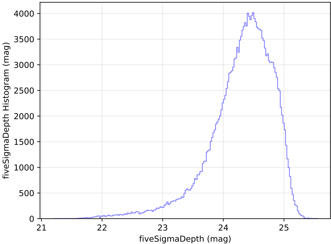
too_elab_r64_d3_griz_v3.4_10yrs g: fiveSigmaDepth Histogram
