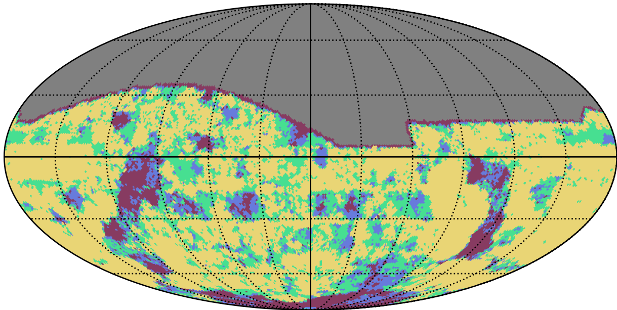
too_elab_r64_d3_griz_v3.4_10yrs g band: YearCoverage night
