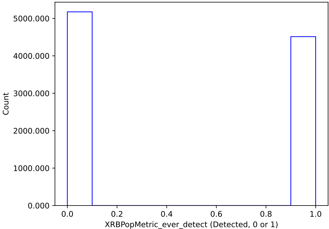
too_elab_r64_d3_griz_v3.4_10yrs : XRBPoMetric_ever_detect
