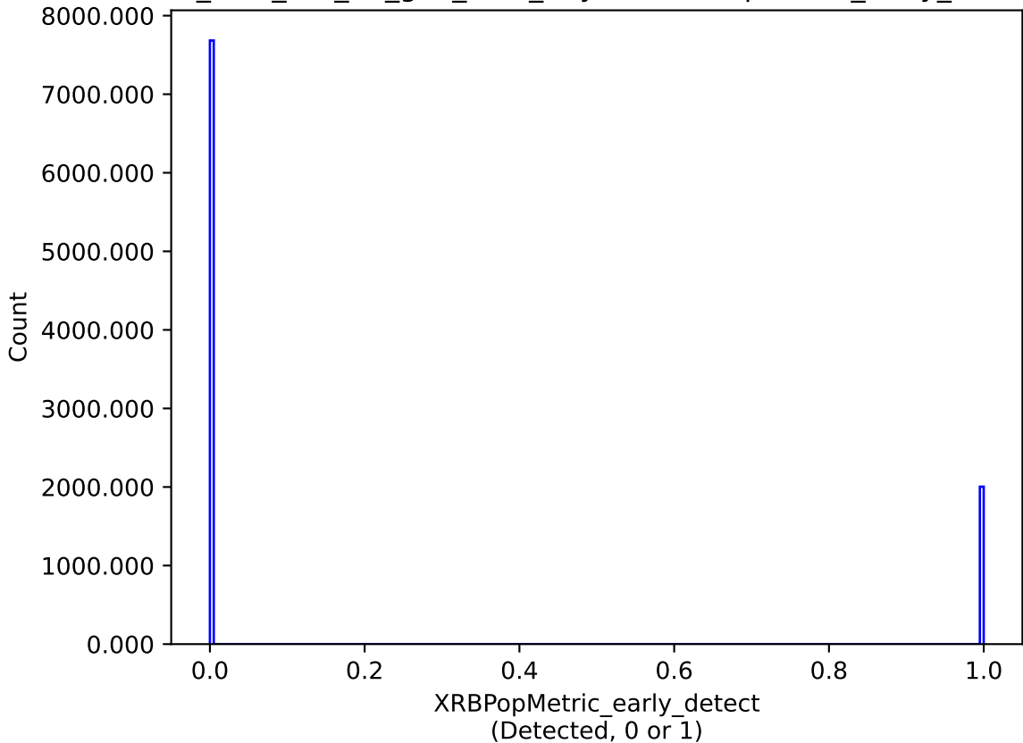
too_elab_r64_d3_griz_v3.4_10yrs : XRBPopMetric_early_detect
