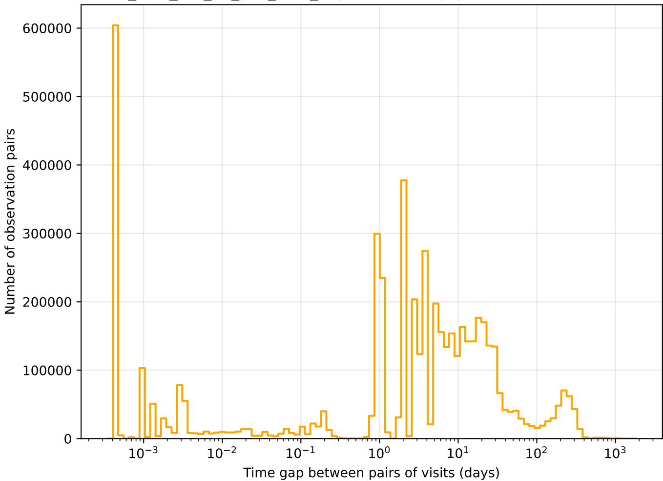
too_elab_r64_d3_griz_v3.4_10yrs r band: Tgaps observationStartMJD
