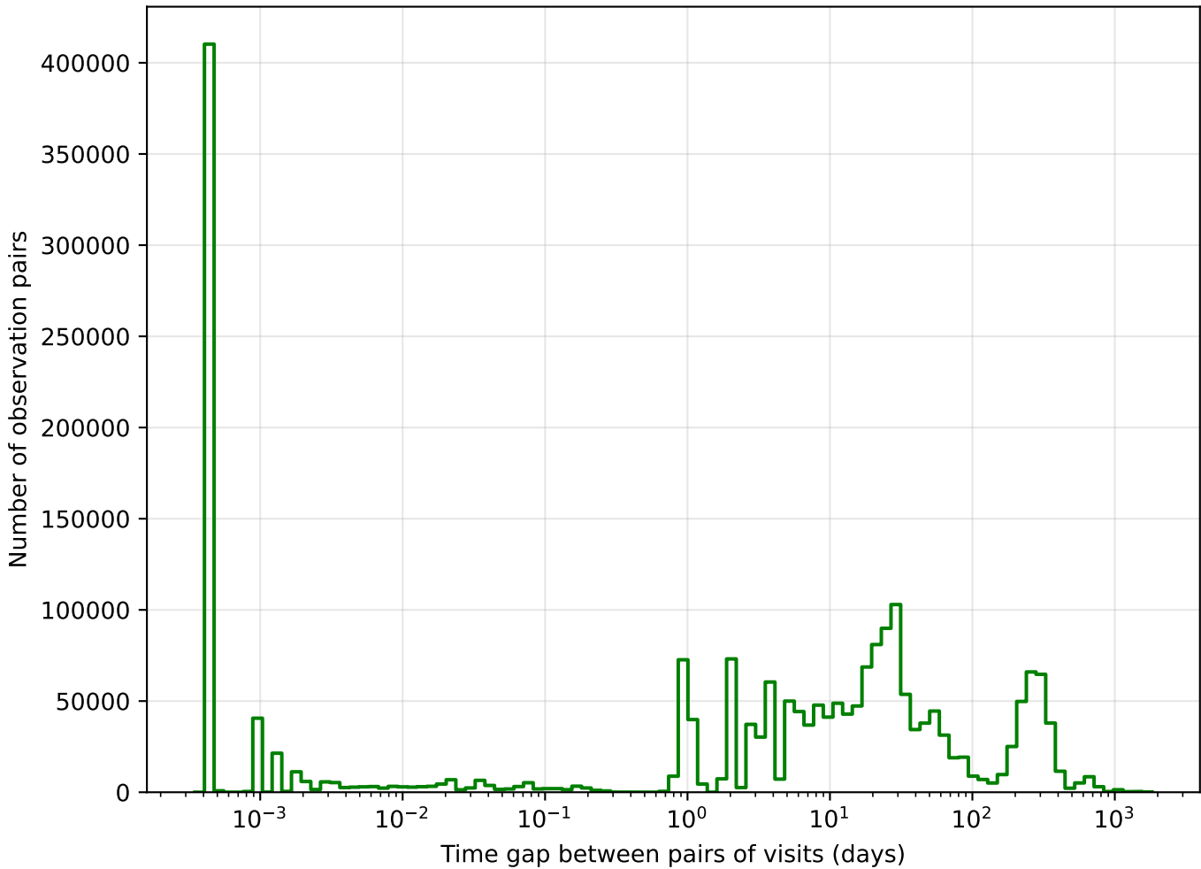
too_elab_r64_d3_griz_v3.4_10yrs g band: Tgaps observationStartMJD
