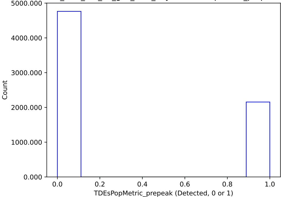
too_elab_r64_d3_griz_v3.4_10yrs : TDEsPopMetric_prepeak
