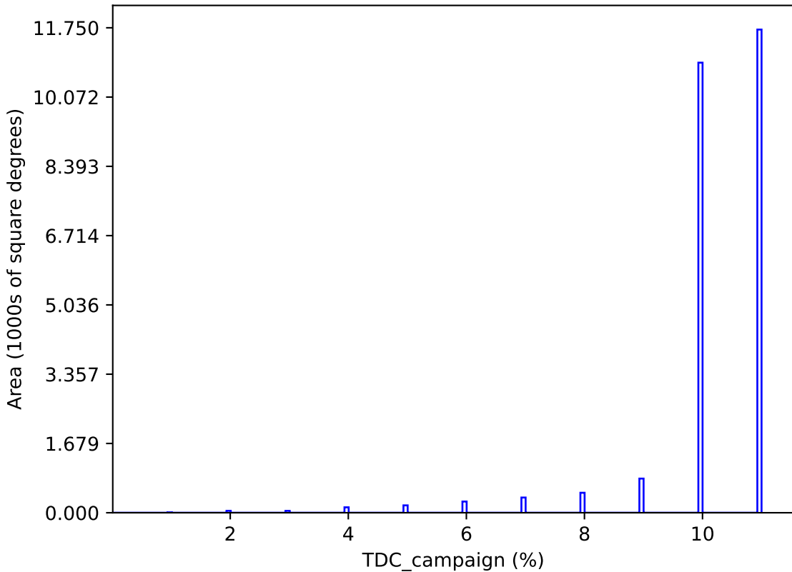
too_elab_r64_d3_griz_v3.4_10yrs : TDC_campaign
