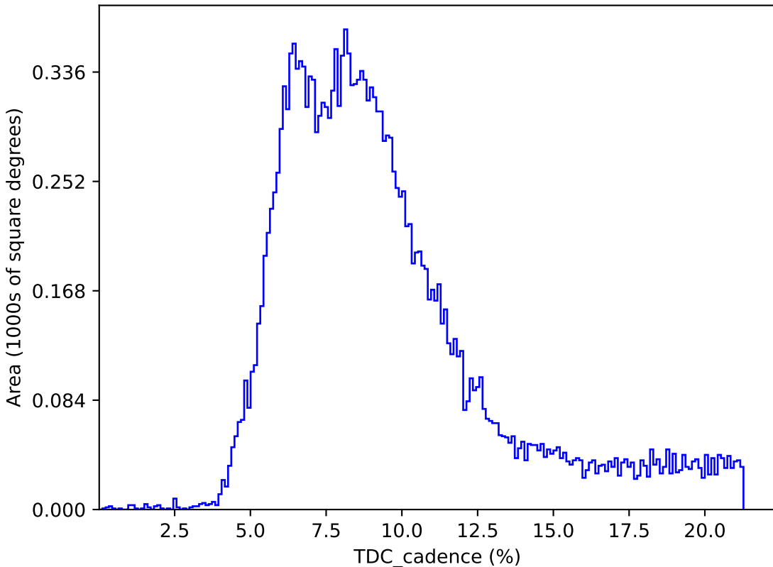
too_elab_r64_d3_griz_v3.4_10yrs : TDC_cadence
