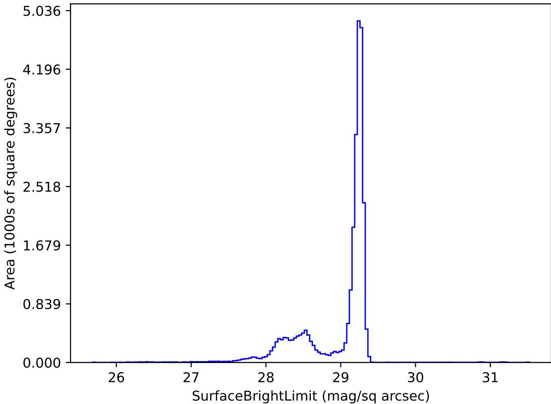
too_elab_r64_d3_griz_v3.4_10yrs z: SurfaceBrightLimit
