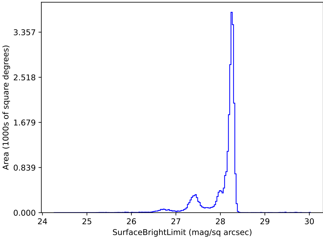
too_elab_r64_d3_griz_v3.4_10yrs y: SurfaceBrightLimit
