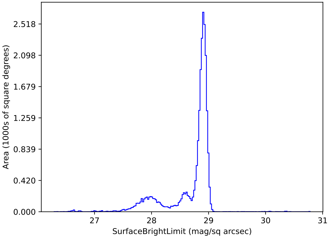
too_elab_r64_d3_griz_v3.4_10yrs u: SurfaceBrightLimit
