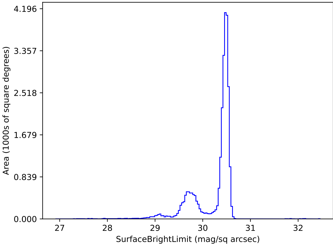
too_elab_r64_d3_griz_v3.4_10yrs r: SurfaceBrightLimit
