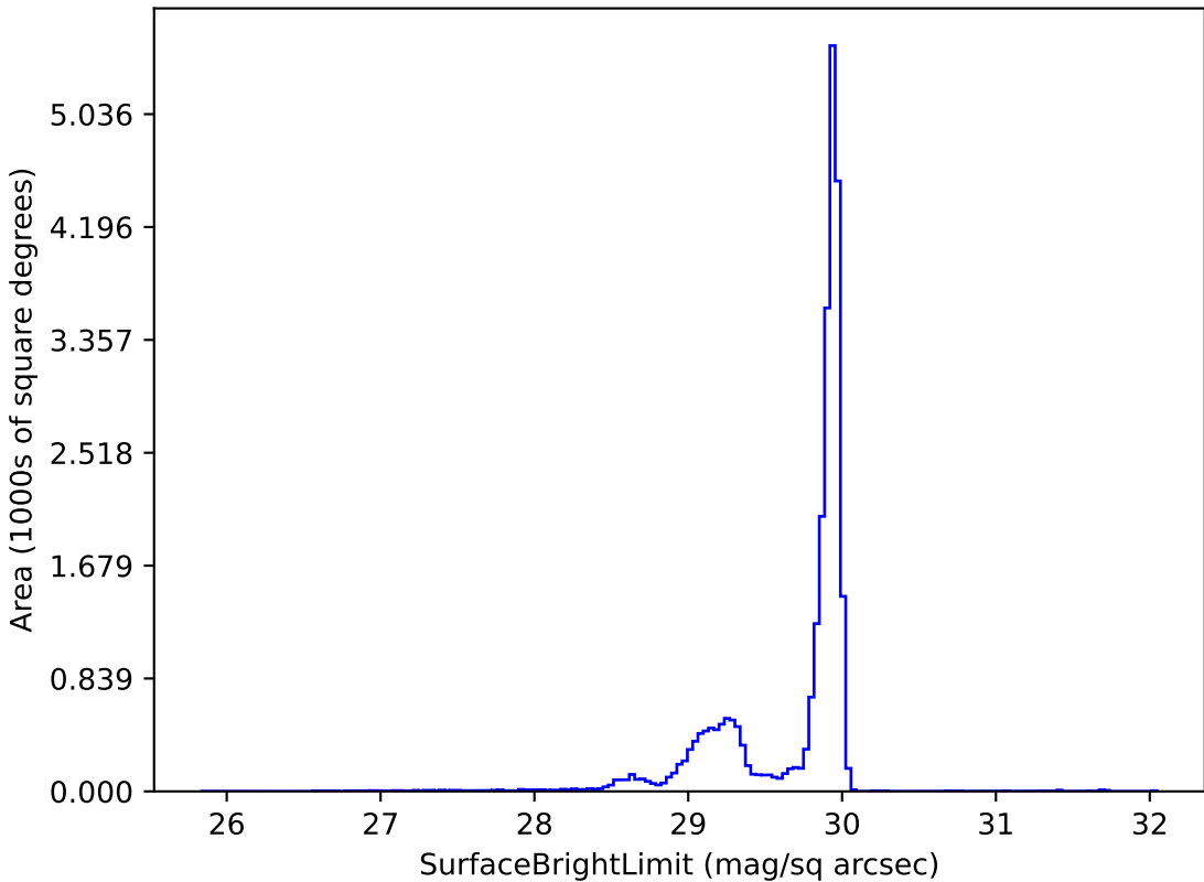
too_elab_r64_d3_griz_v3.4_10yrs i: SurfaceBrightLimit
