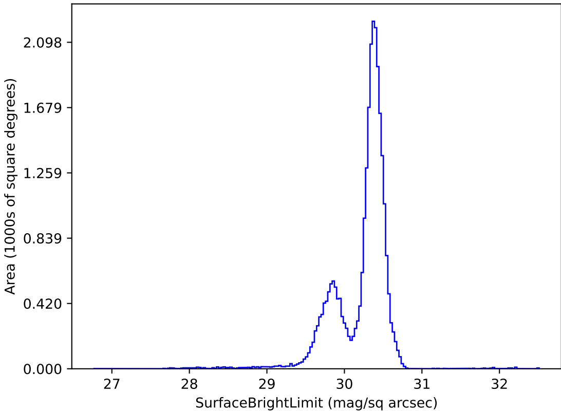
too_elab_r64_d3_griz_v3.4_10yrs g: SurfaceBrightLimit
