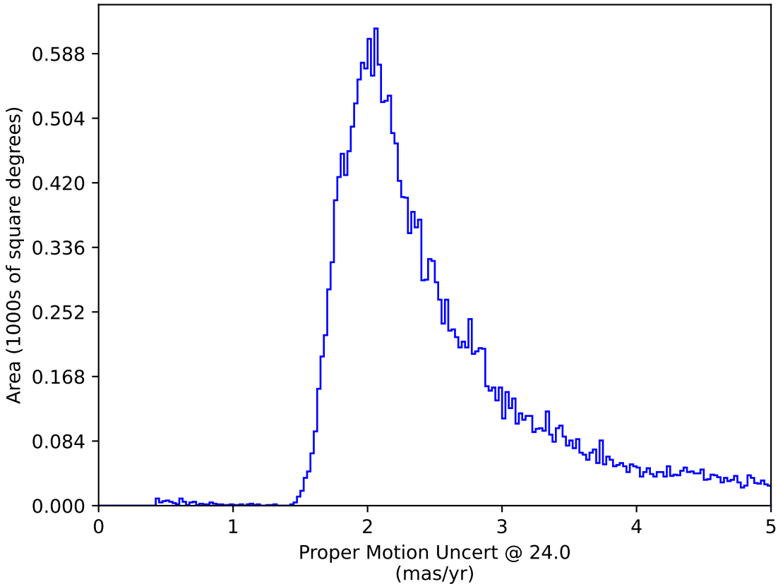
too_elab_r64_d3_griz_v3.4_10yrs : Proper Motion Uncert @ 24.0
