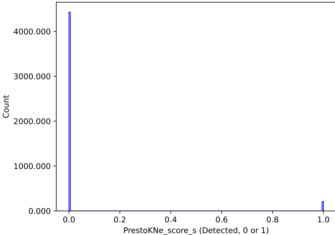
too_elab_r64_d3_griz_v3.4_10yrs : PrestoKNe_score_s
