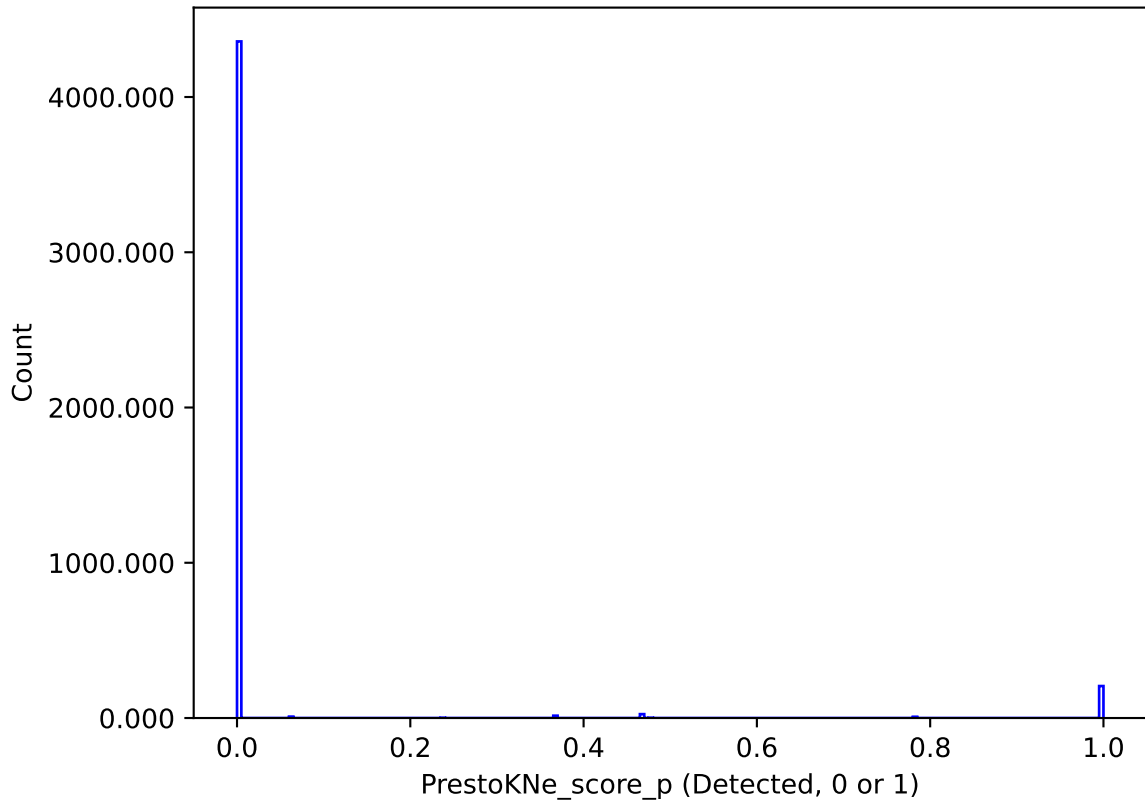
too_elab_r64_d3_griz_v3.4_10yrs : PrestoKNe_score_p
