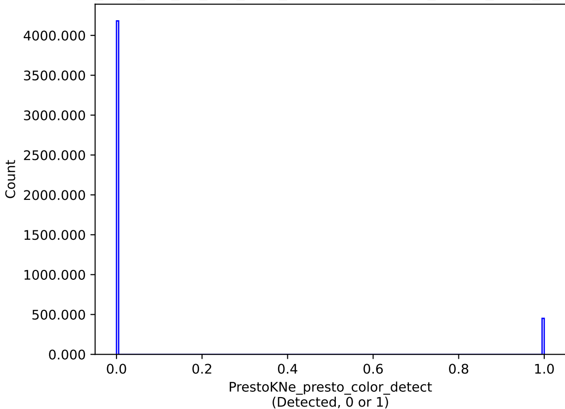
too_elab_r64_d3_griz_v3.4_10yrs : PrestoKNe_presto_color_detect
