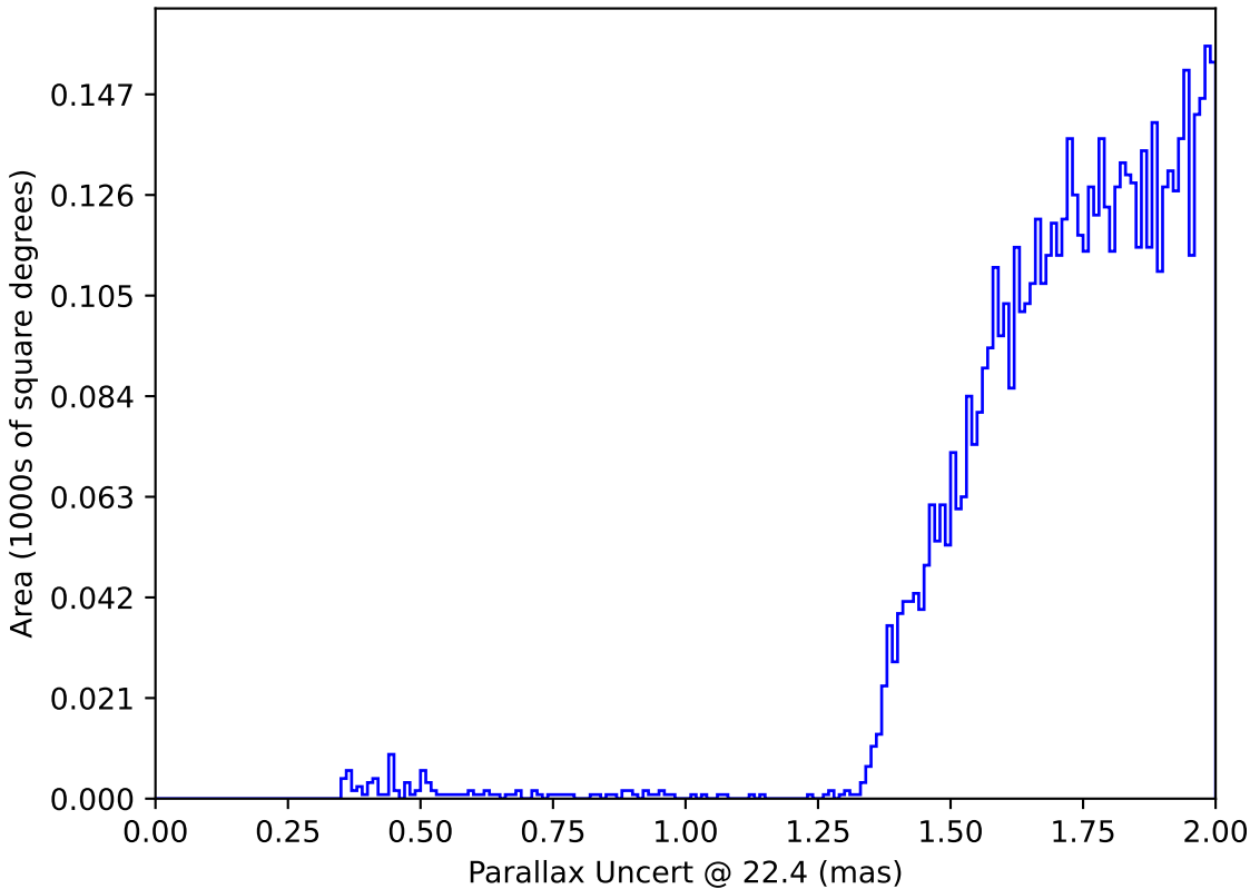
too_elab_r64_d3_griz_v3.4_10yrs : Parallax Uncert @ 22.4
