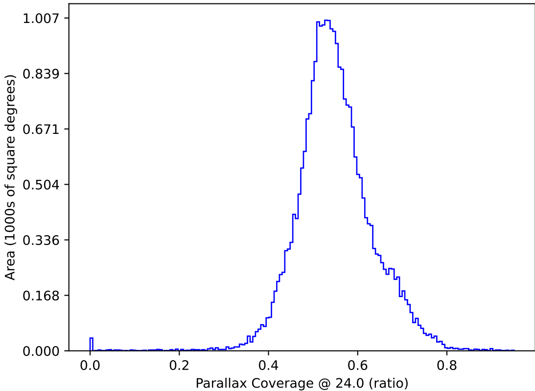
too_elab_r64_d3_griz_v3.4_10yrs : Parallax Coverage @ 24.0
