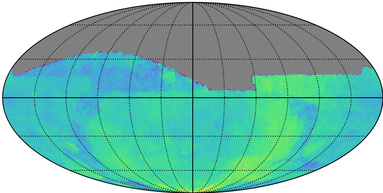
too_elab_r64_d3_griz_v3.4_10yrs : Parallax Coverage @ 22.4
