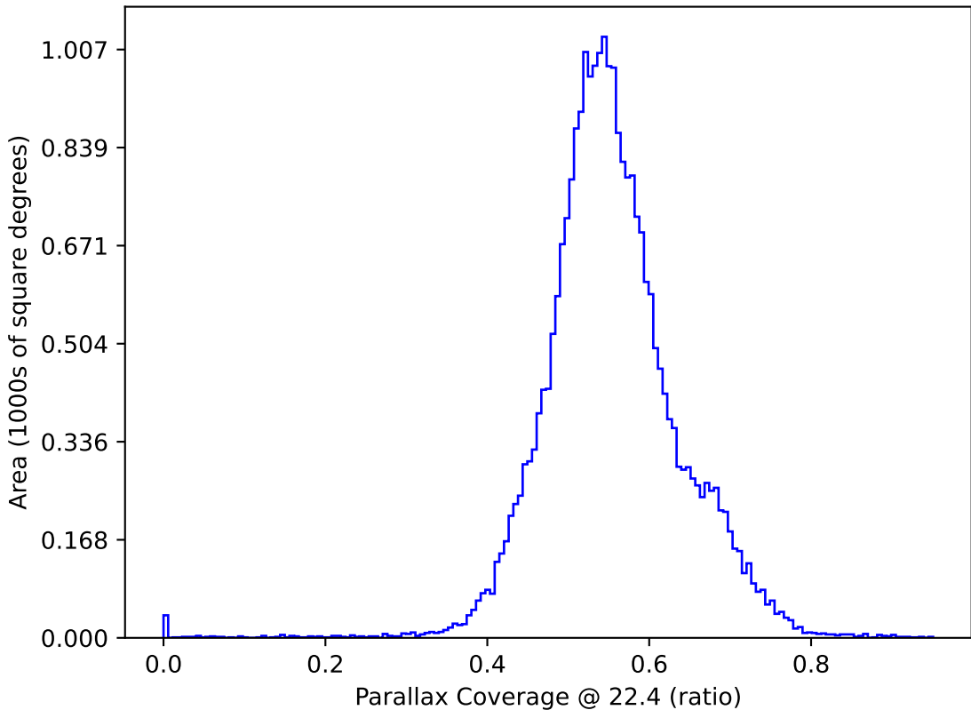
too_elab_r64_d3_griz_v3.4_10yrs : Parallax Coverage @ 22.4
