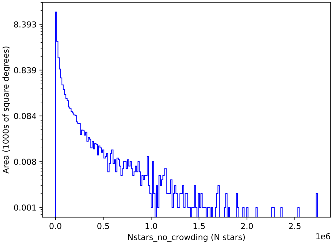
too_elab_r64_d3_griz_v3.4_10yrs u: Nstars_no_crowding
