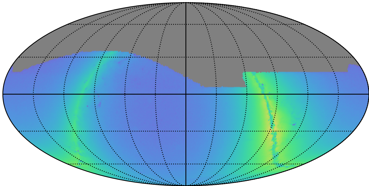
too_elab_r64_d3_griz_v3.4_10yrs r: Nstars_no_crowding
