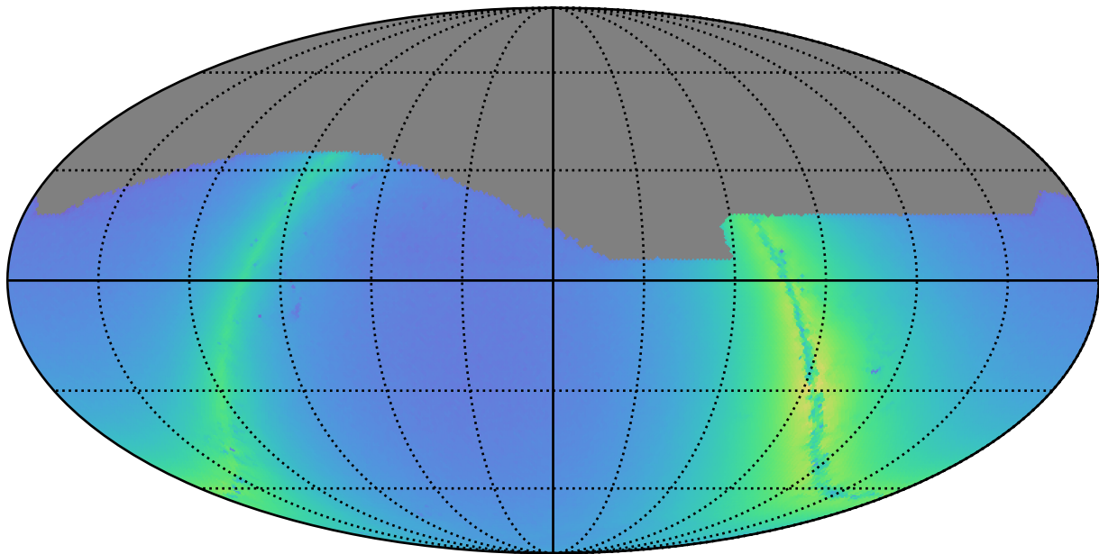
too_elab_r64_d3_griz_v3.4_10yrs i: Nstars_no_crowding
