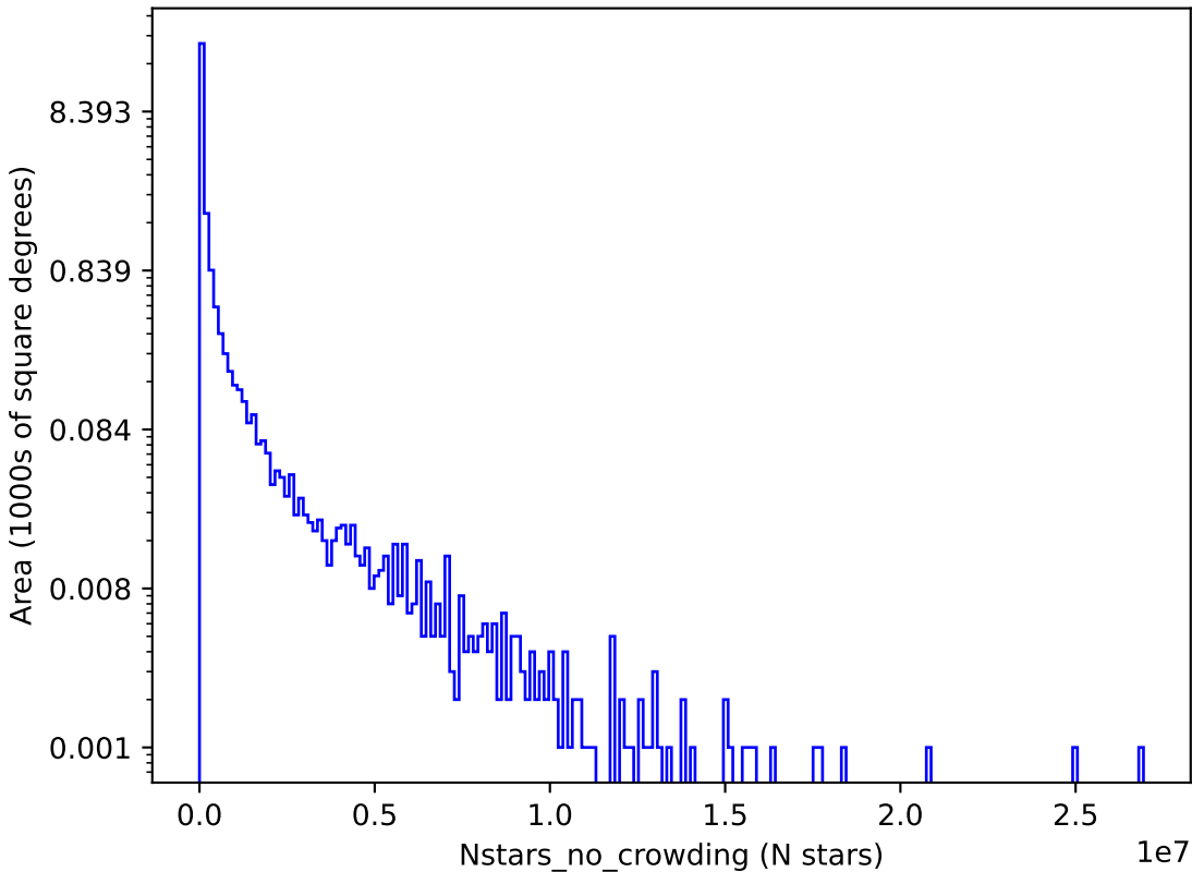
too_elab_r64_d3_griz_v3.4_10yrs i: Nstars_no_crowding
