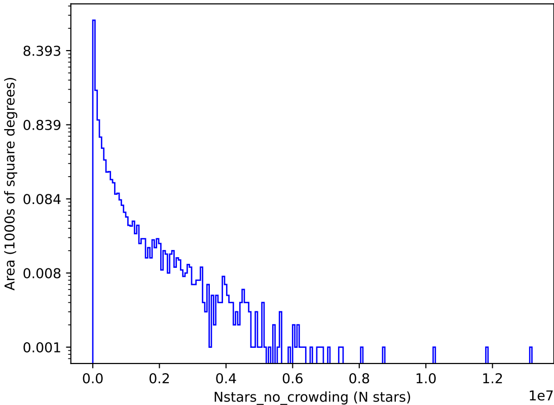
too_elab_r64_d3_griz_v3.4_10yrs g: Nstars_no_crowding
