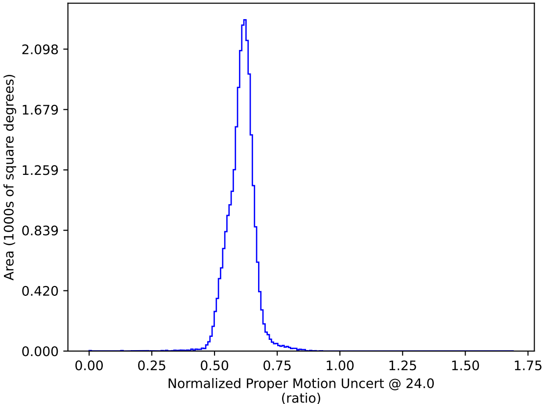
too_elab_r64_d3_griz_v3.4_10yrs : Normalized Proper Motion Uncert @ 24.0
