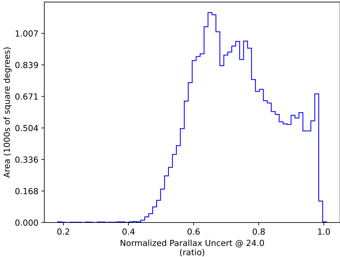
too_elab_r64_d3_griz_v3.4_10yrs : Normalized Parallax Uncert @ 24.0
