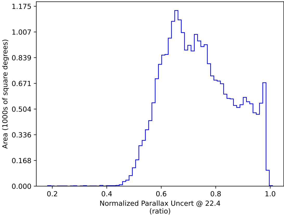
too_elab_r64_d3_griz_v3.4_10yrs : Normalized Parallax Uncert @ 22.4
