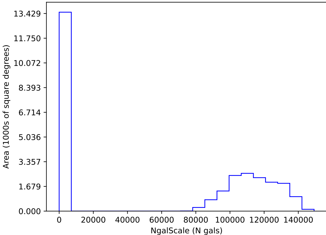
too_elab_r64_d3_griz_v3.4_10yrs i: NgalScale
