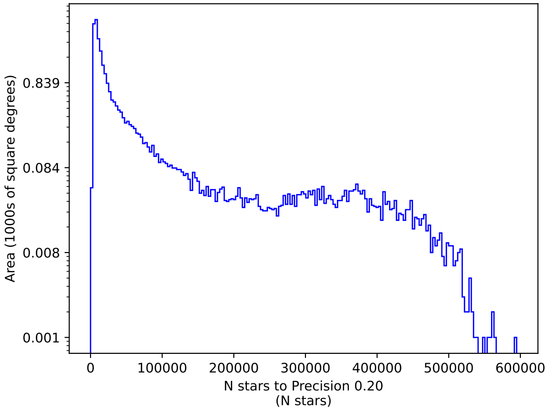
too_elab_r64_d3_griz_v3.4_10yrs g: N stars to Precision 0.20
