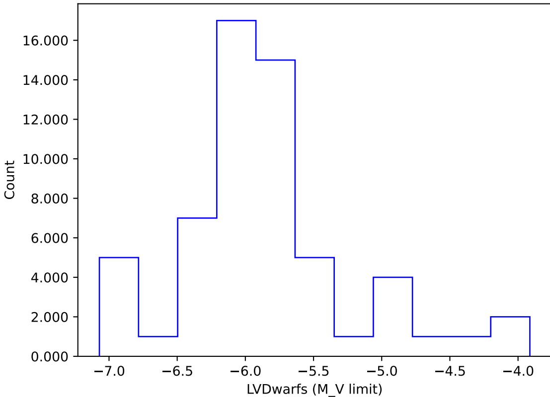
too_elab_r64_d3_griz_v3.4_10yrs gi: LVDwarfs
