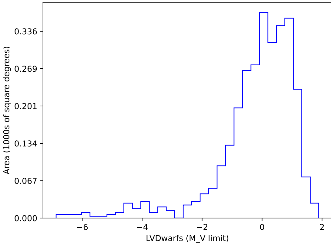
too_elab_r64_d3_griz_v3.4_10yrs gi SCP: LVDwarfs
