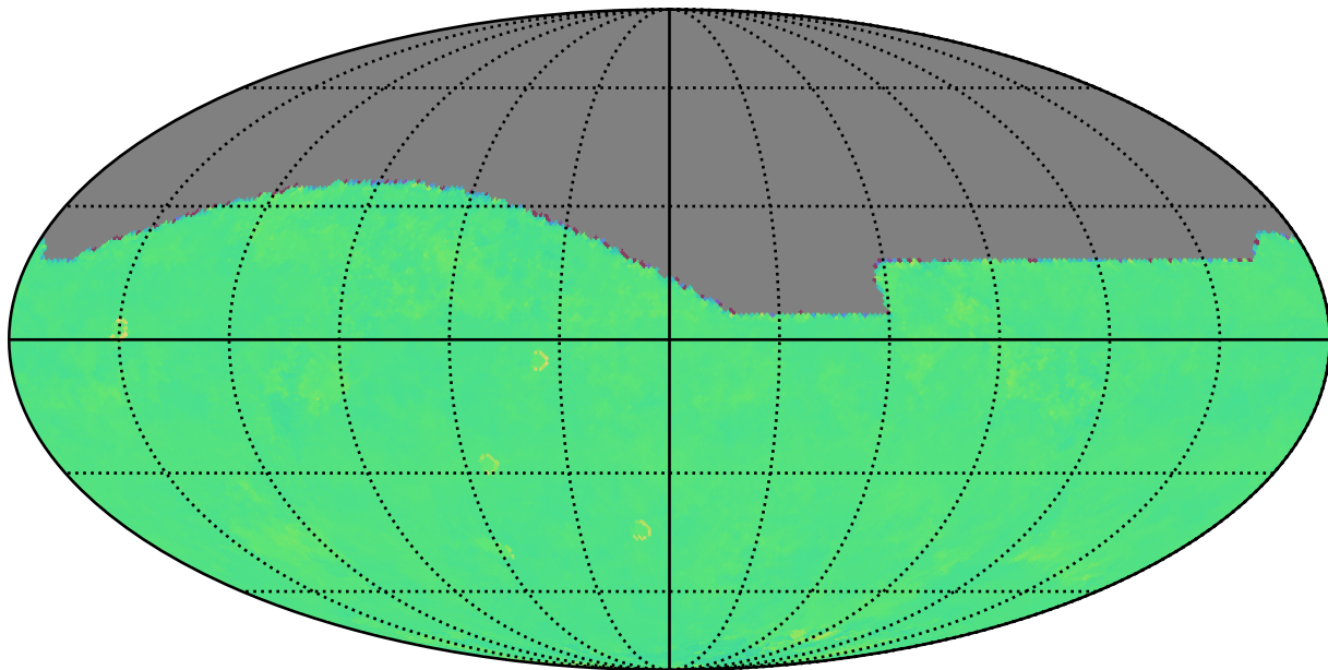
too_elab_r64_d3_griz_v3.4_10yrs r: Kuiper rotTelPos
