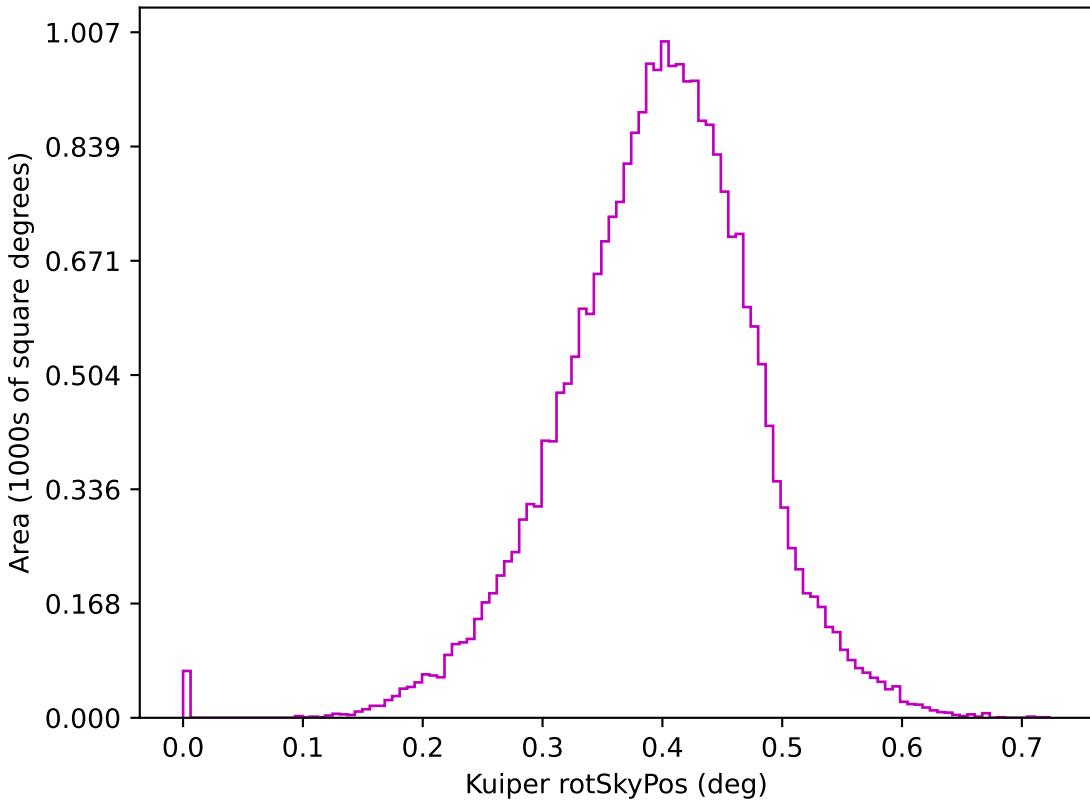
too_elab_r64_d3_griz_v3.4_10yrs z: Kuiper rotSkyPos
