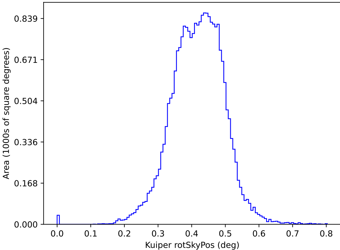
too_elab_r64_d3_griz_v3.4_10yrs y: Kuiper rotSkyPos
