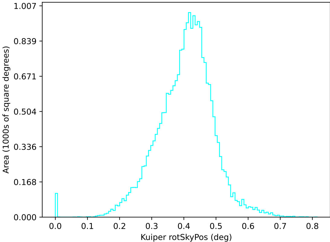
too_elab_r64_d3_griz_v3.4_10yrs u: Kuiper rotSkyPos
